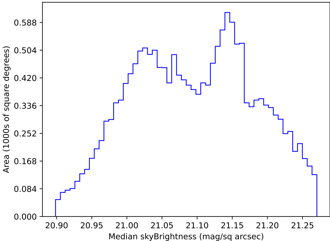
extra_ss_neo7_v3.4_10yrs WFD r band: Median skyBrightness
