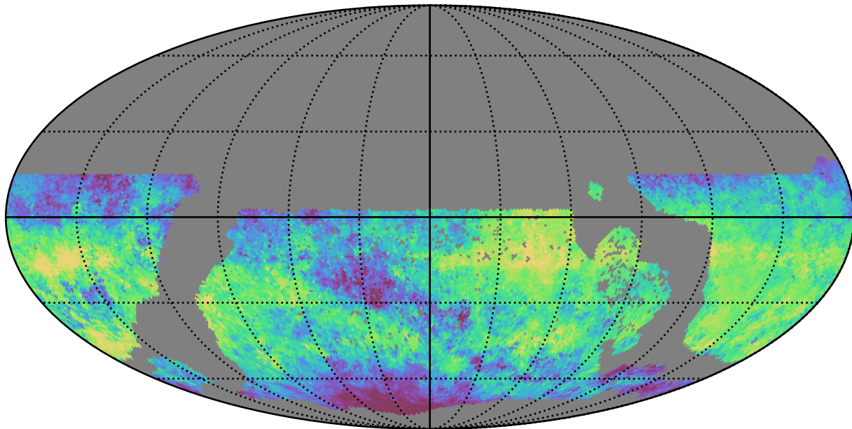
extra_ss_neo7_v3.4_10yrs WFD i band: Median skyBrightness
