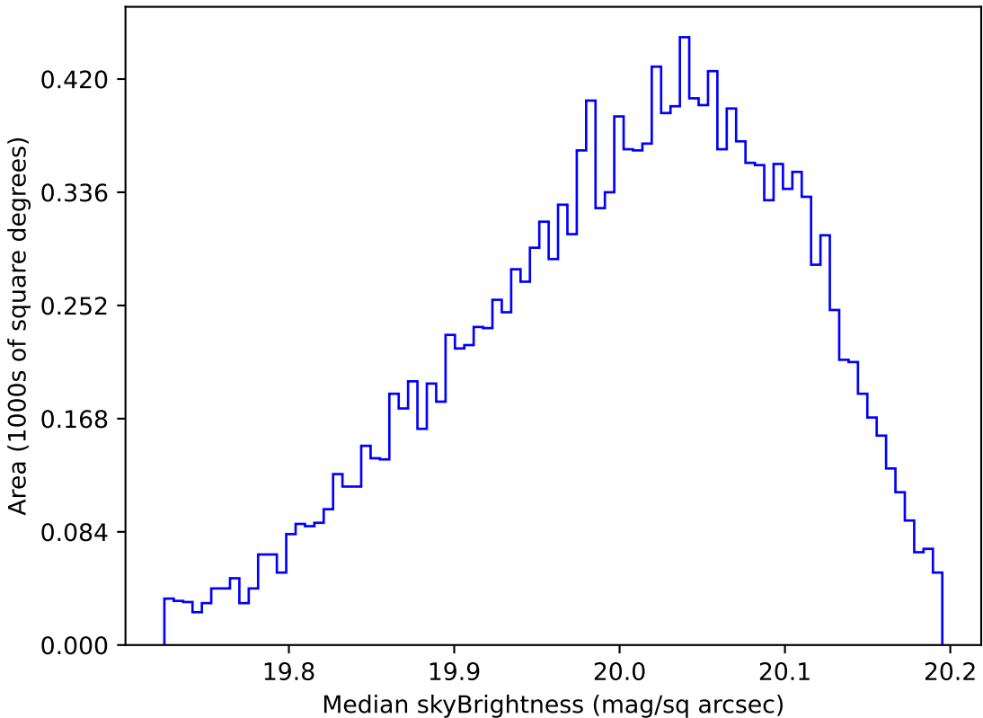
extra_ss_neo7_v3.4_10yrs WFD i band: Median skyBrightness
