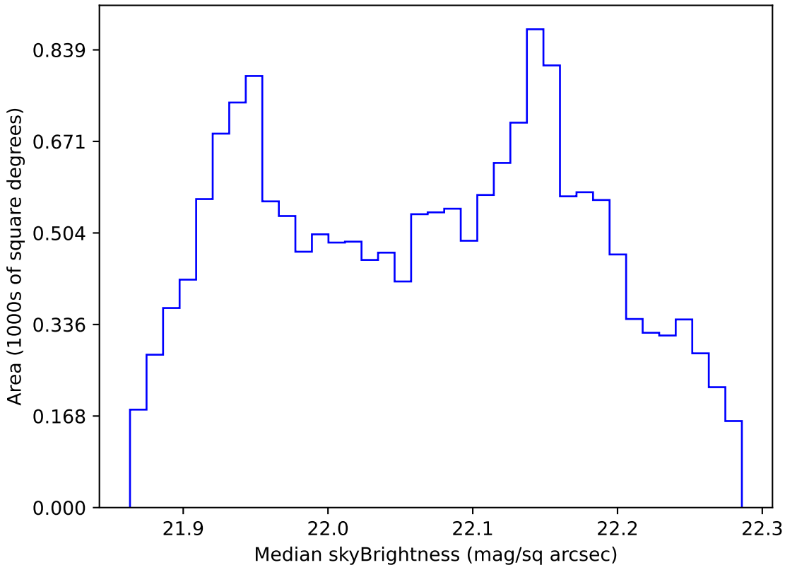
extra_ss_neo7_v3.4_10yrs WFD g band: Median skyBrightness
