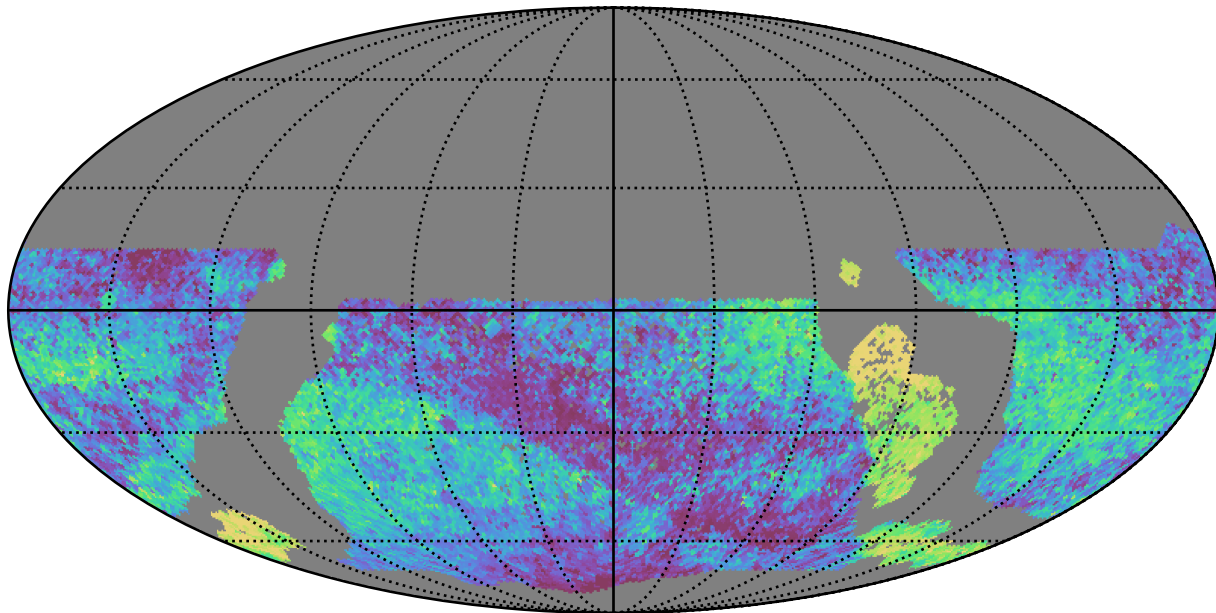
extra_ss_neo7_v3.4_10yrs WFD all bands: Median skyBrightness
