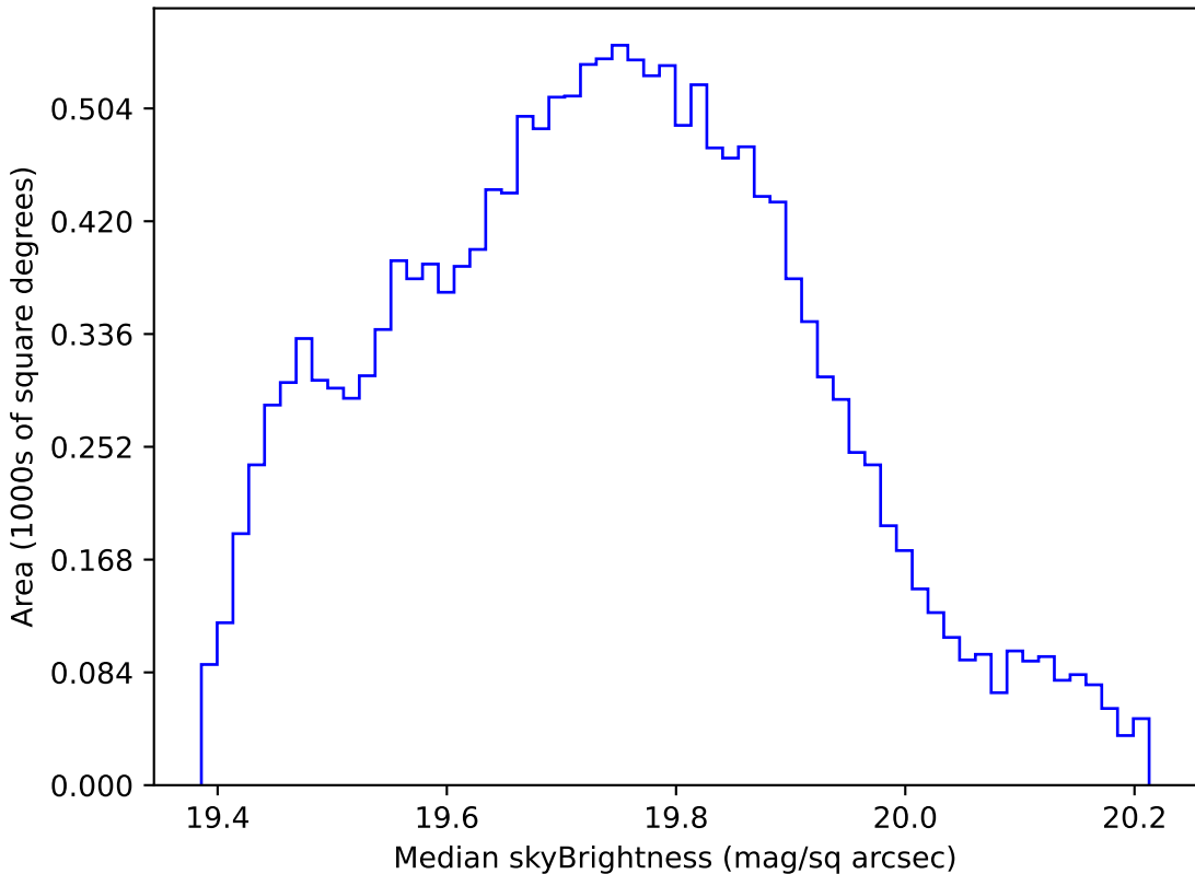
extra_ss_neo7_v3.4_10yrs WFD all bands: Median skyBrightness
