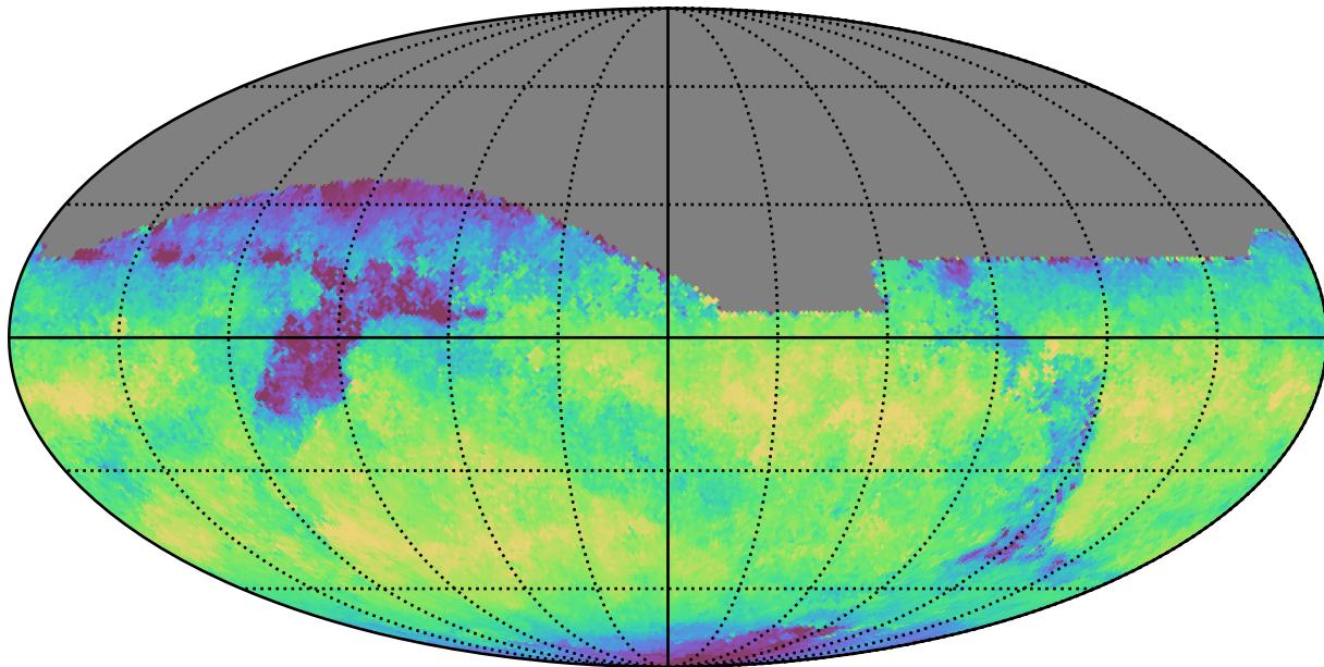
extra_ss_neo7_v3.4_10yrs All sky z band: Median skyBrightness
