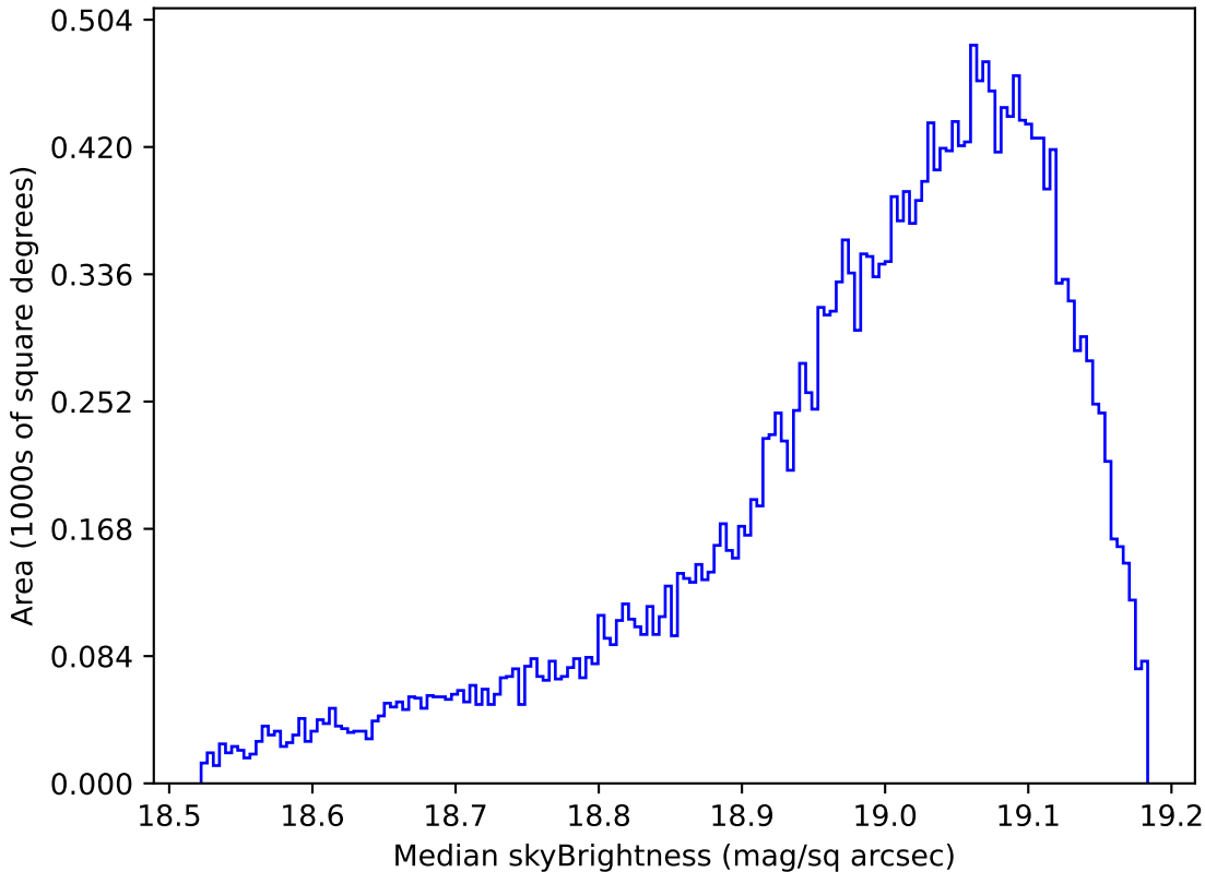
extra_ss_neo7_v3.4_10yrs All sky z band: Median skyBrightness
