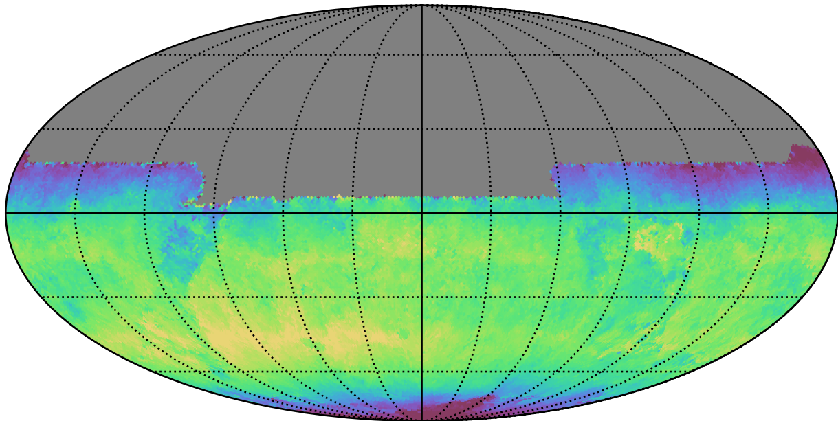
extra_ss_neo7_v3.4_10yrs All sky y band: Median skyBrightness
