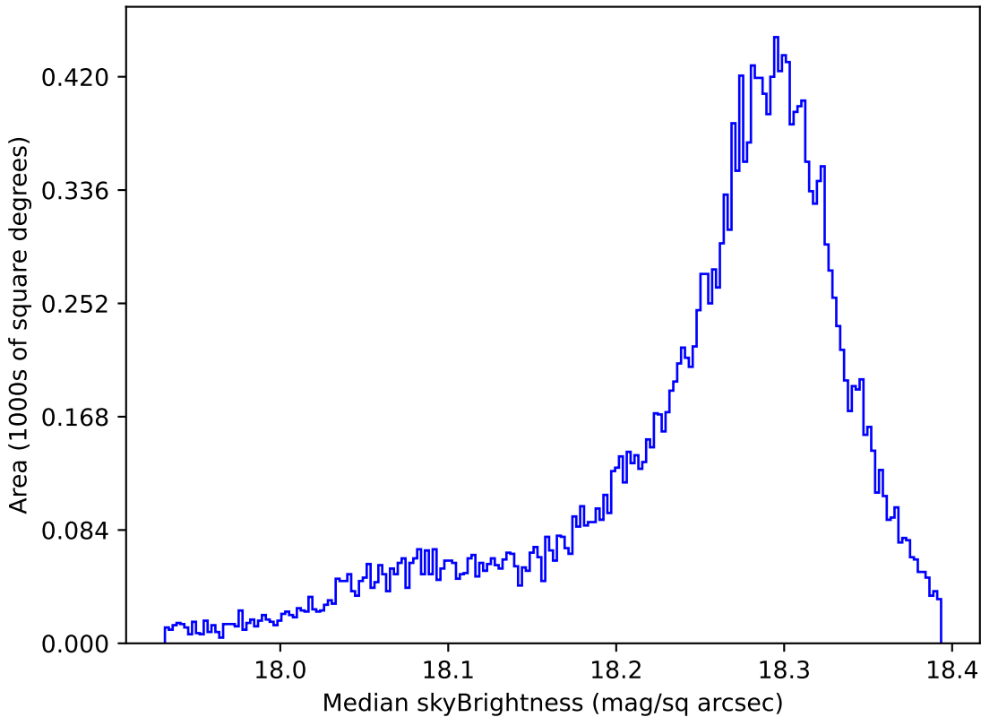
extra_ss_neo7_v3.4_10yrs All sky y band: Median skyBrightness
