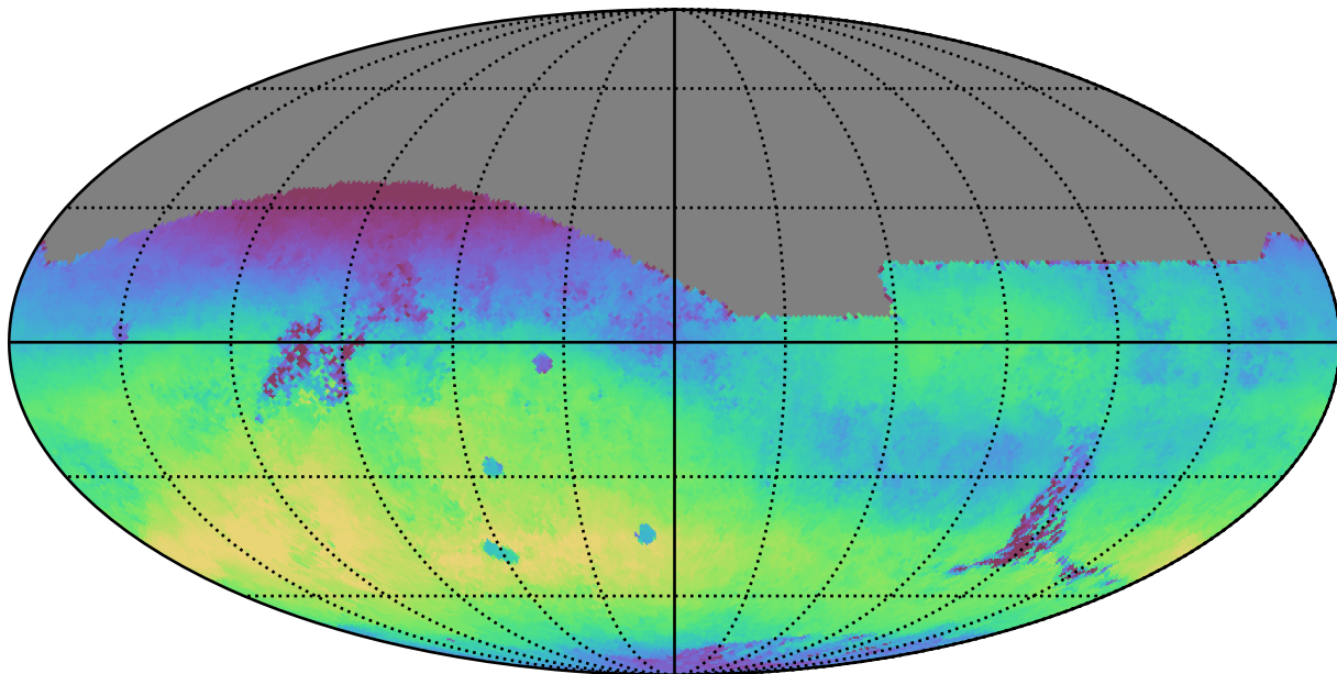
extra_ss_neo7_v3.4_10yrs All sky r band: Median skyBrightness
