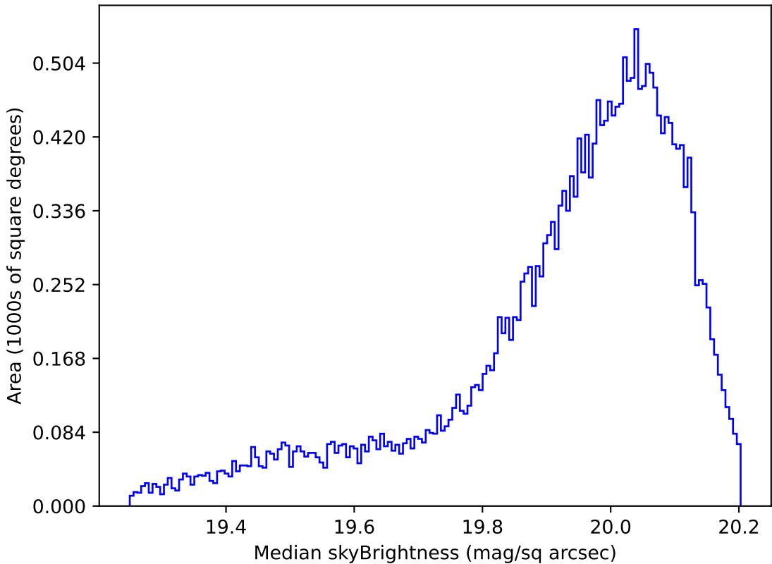
extra_ss_neo7_v3.4_10yrs All sky i band: Median skyBrightness
