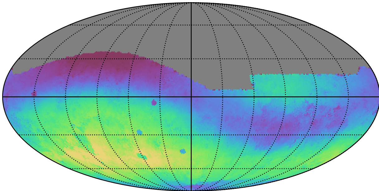
extra_ss_neo7_v3.4_10yrs All sky g band: Median skyBrightness
