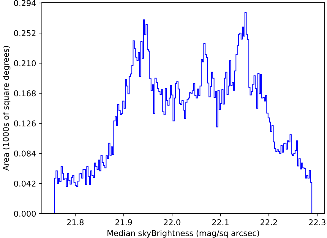
extra_ss_neo7_v3.4_10yrs All sky g band: Median skyBrightness
