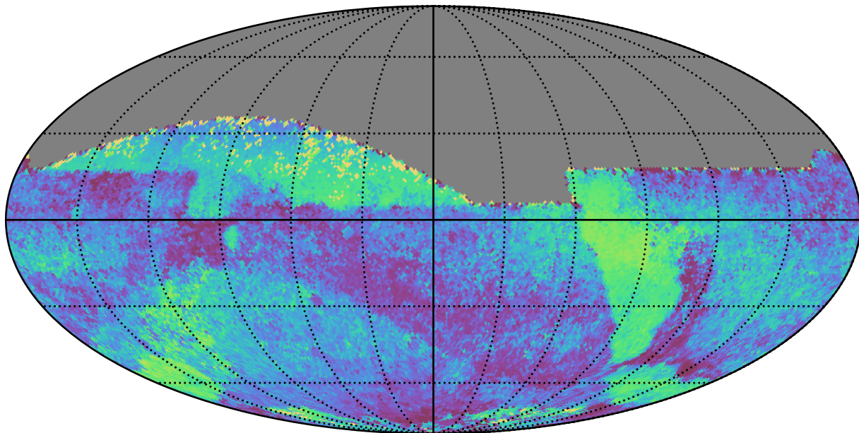
extra_ss_neo7_v3.4_10yrs All sky all bands: Median skyBrightness
