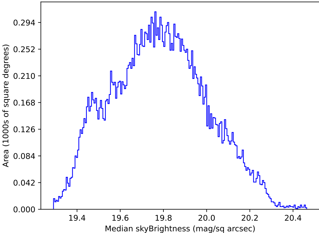
extra_ss_neo7_v3.4_10yrs All sky all bands: Median skyBrightness
