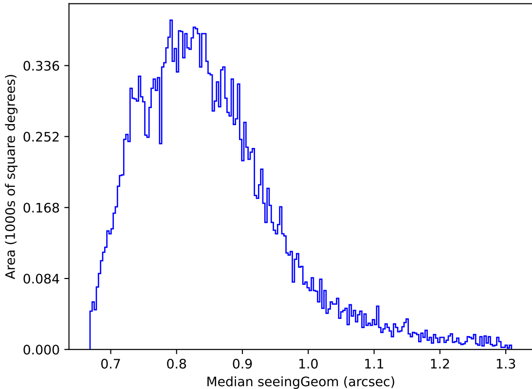
extra_ss_neo7_v3.4_10yrs Yr 1 z band: Median seeingGeom
