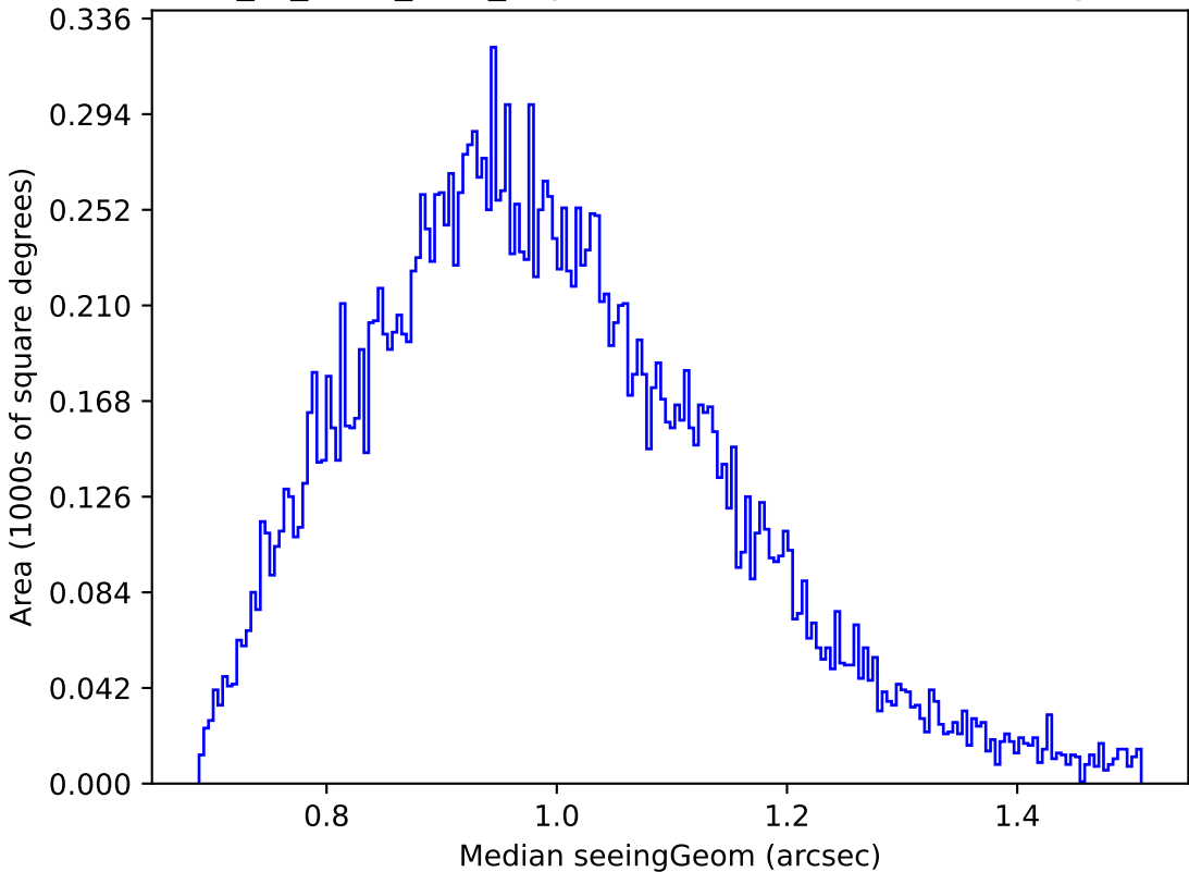
extra_ss_neo7_v3.4_10yrs Yr 1 u band: Median seeingGeom
