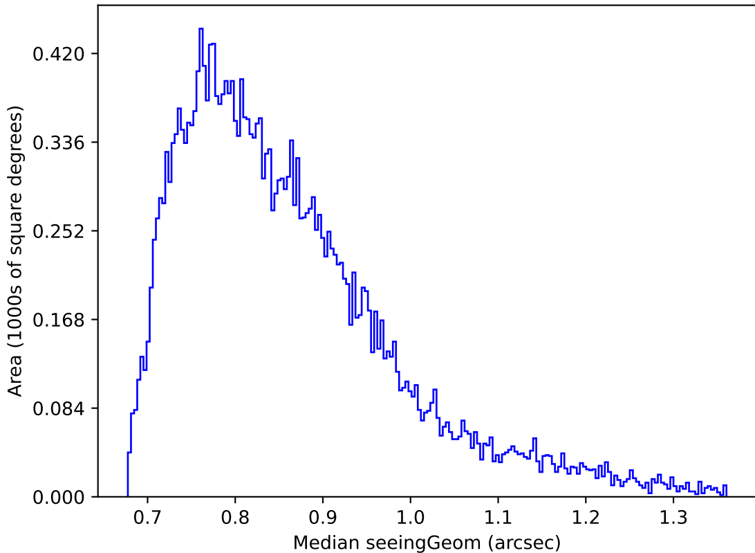
extra_ss_neo7_v3.4_10yrs Yr 1 r band: Median seeingGeom
