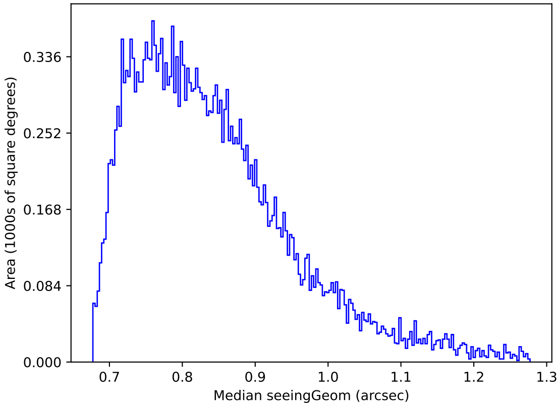
extra_ss_neo7_v3.4_10yrs Yr 1 i band: Median seeingGeom
