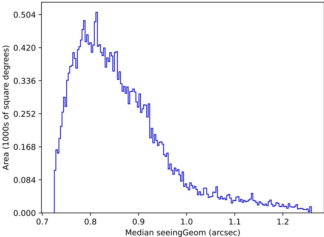
extra_ss_neo7_v3.4_10yrs Yr 1 all bands: Median seeingGeom
