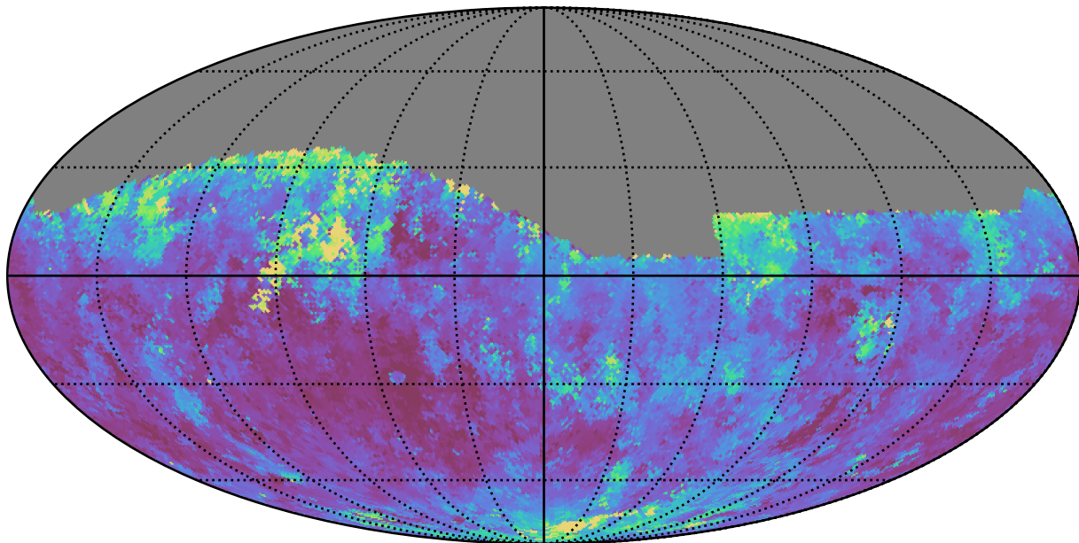
extra_ss_neo7_v3.4_10yrs Yr 1 z band: Median seeingEff
