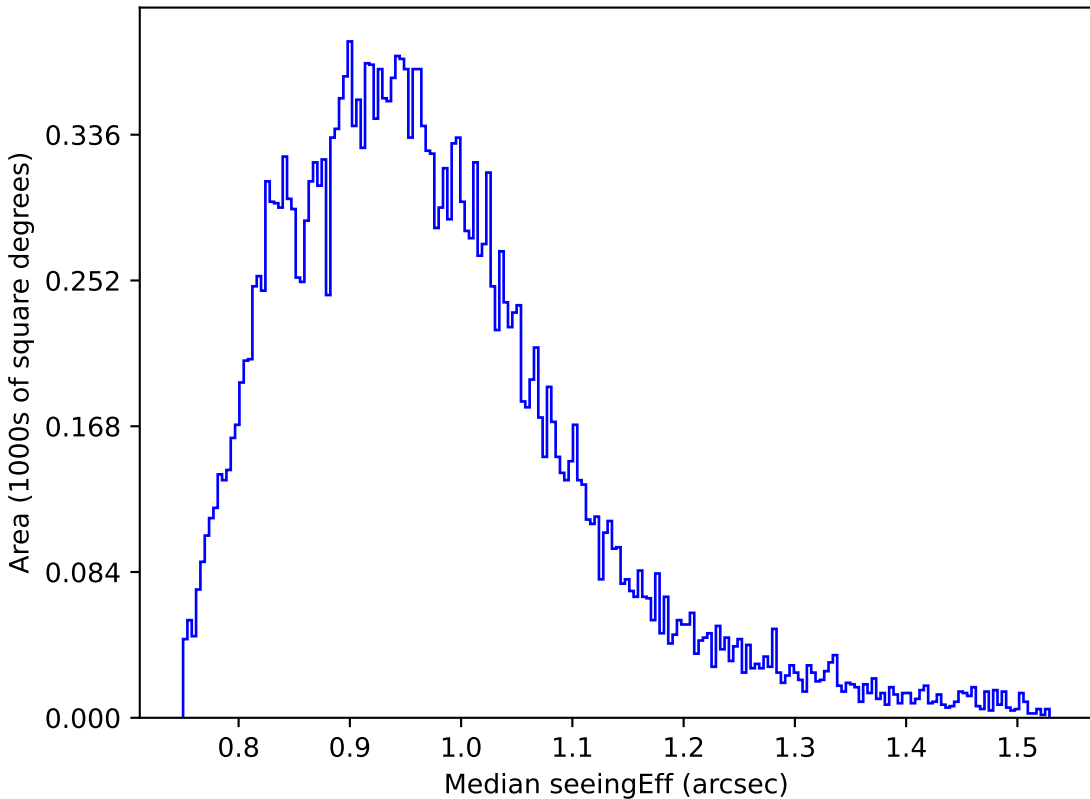
extra_ss_neo7_v3.4_10yrs Yr 1 z band: Median seeingEff
