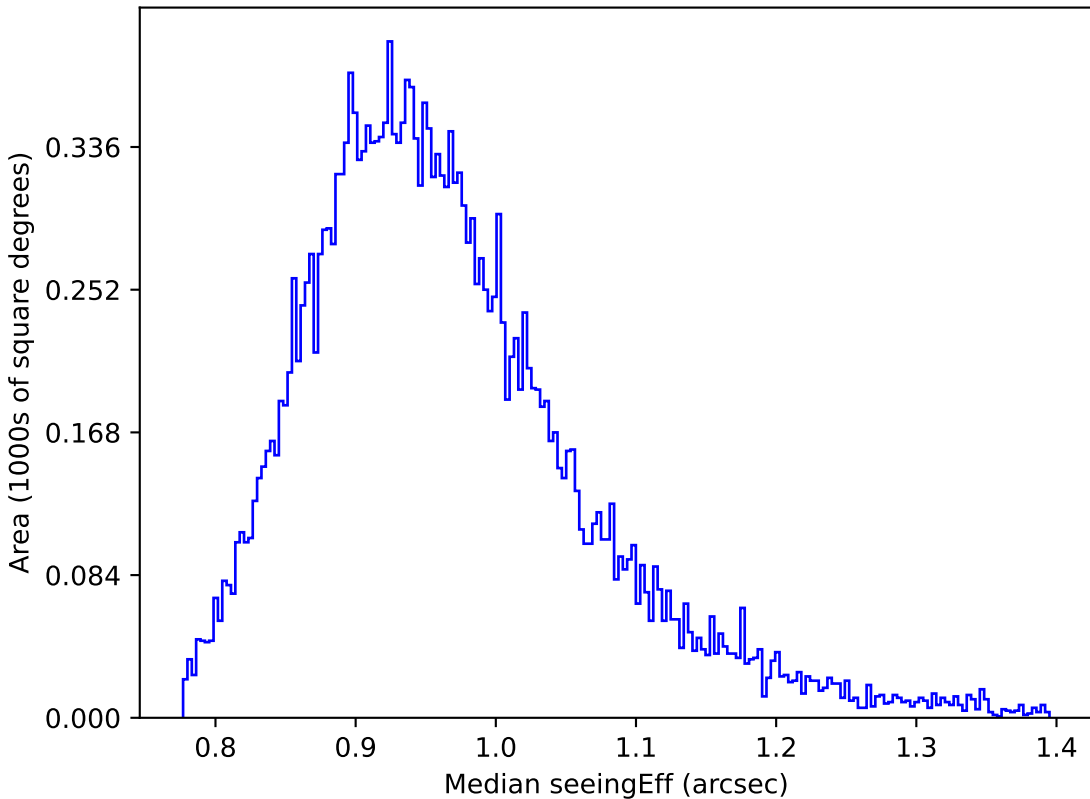
extra_ss_neo7_v3.4_10yrs Yr 1 y band: Median seeingEff
