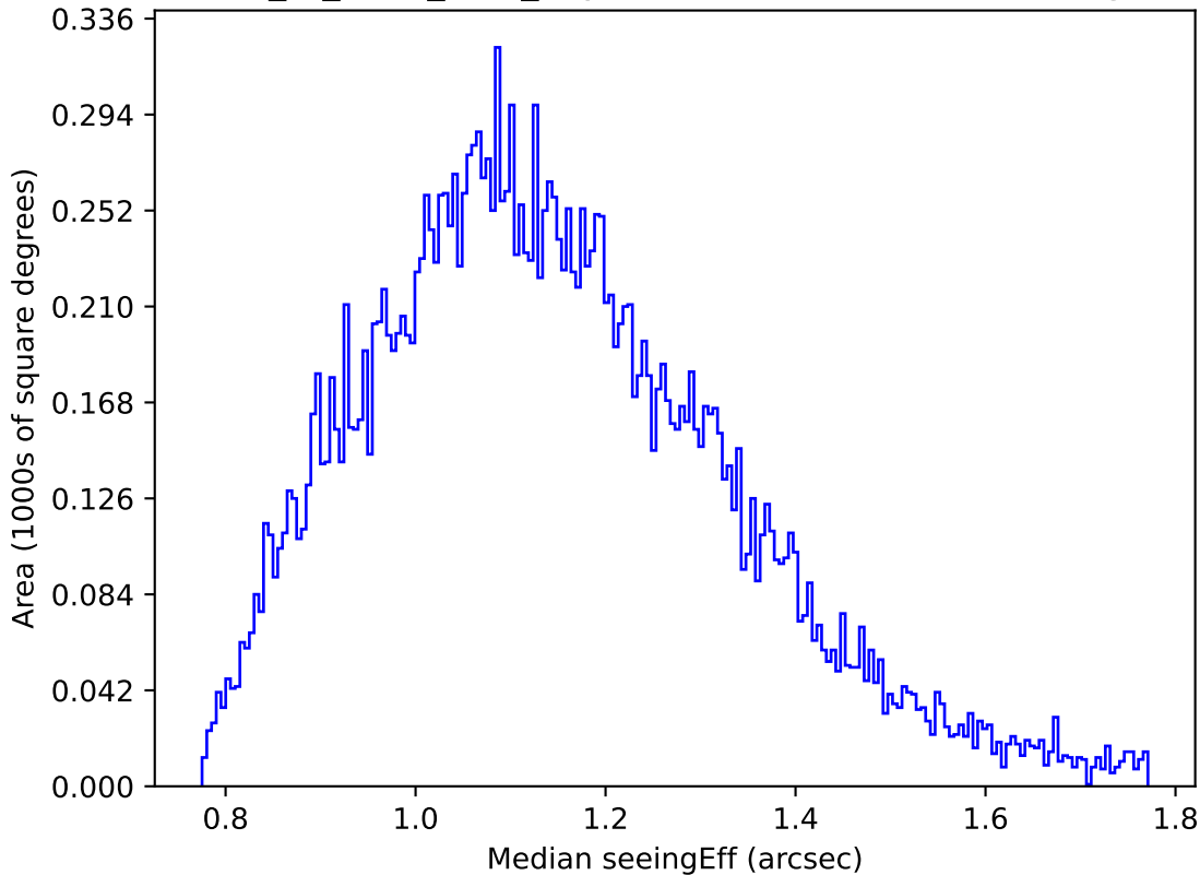
extra_ss_neo7_v3.4_10yrs Yr 1 u band: Median seeingEff
