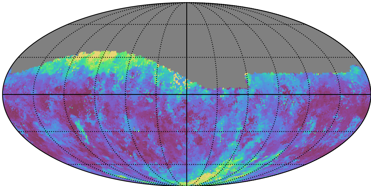
extra_ss_neo7_v3.4_10yrs Yr 1 g band: Median seeingEff
