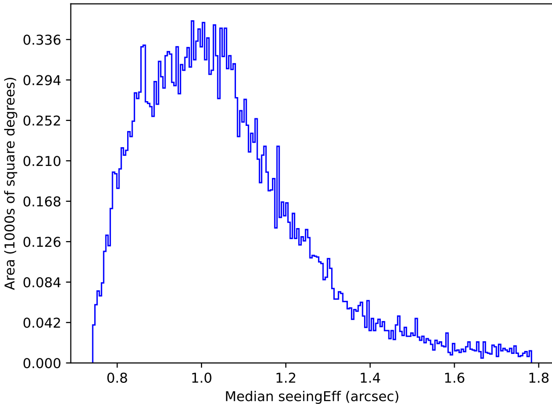
extra_ss_neo7_v3.4_10yrs Yr 1 g band: Median seeingEff
