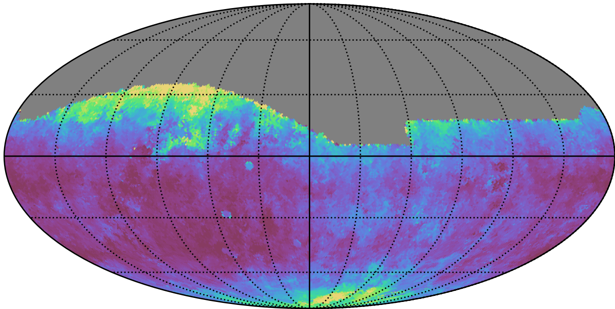
extra_ss_neo7_v3.4_10yrs Yr 1 all bands: Median seeingEff
