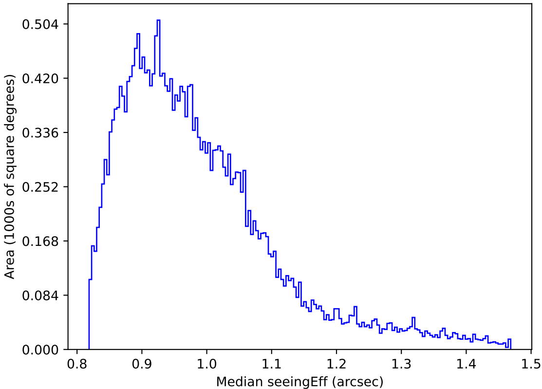
extra_ss_neo7_v3.4_10yrs Yr 1 all bands: Median seeingEff
