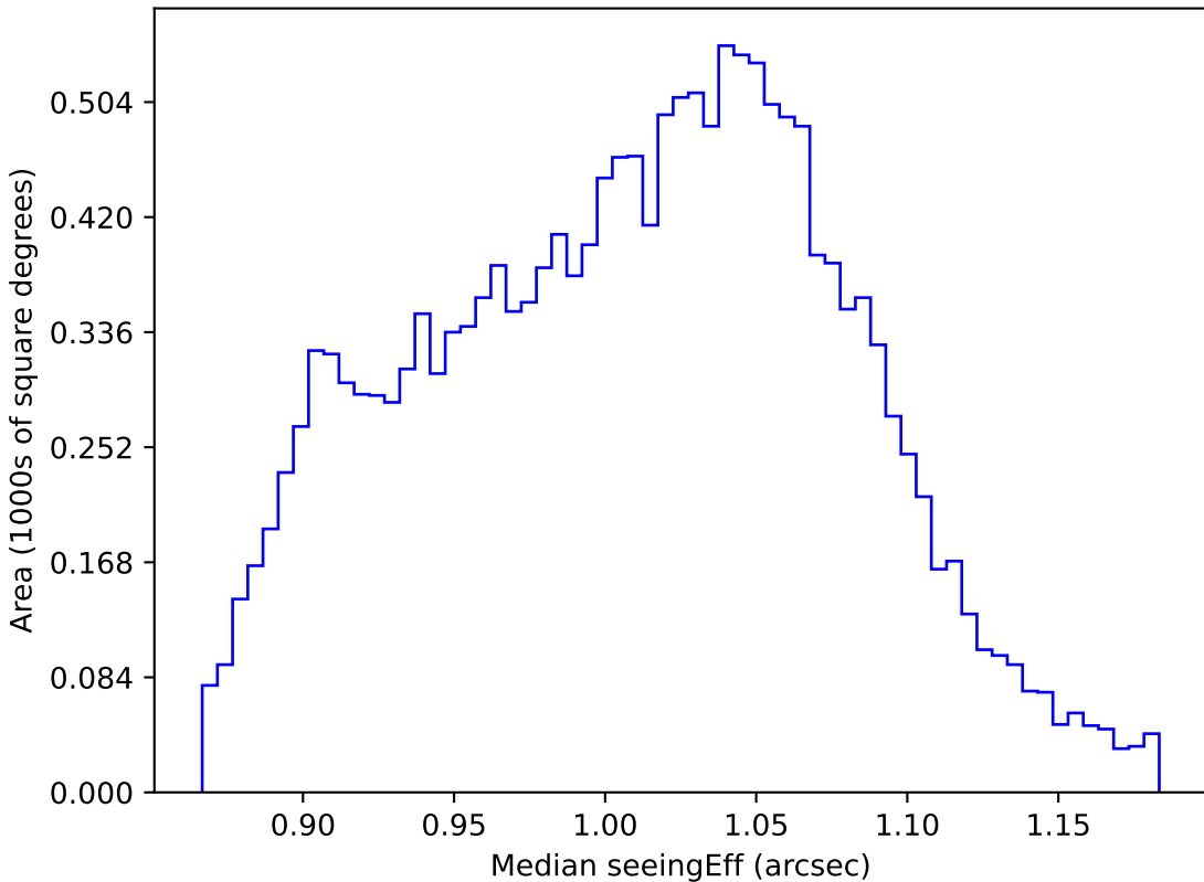
extra_ss_neo7_v3.4_10yrs WFD z band: Median seeingEff
