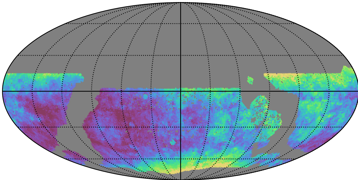
extra_ss_neo7_v3.4_10yrs WFD y band: Median seeingEff
