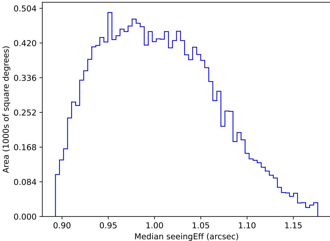
extra_ss_neo7_v3.4_10yrs WFD y band: Median seeingEff
