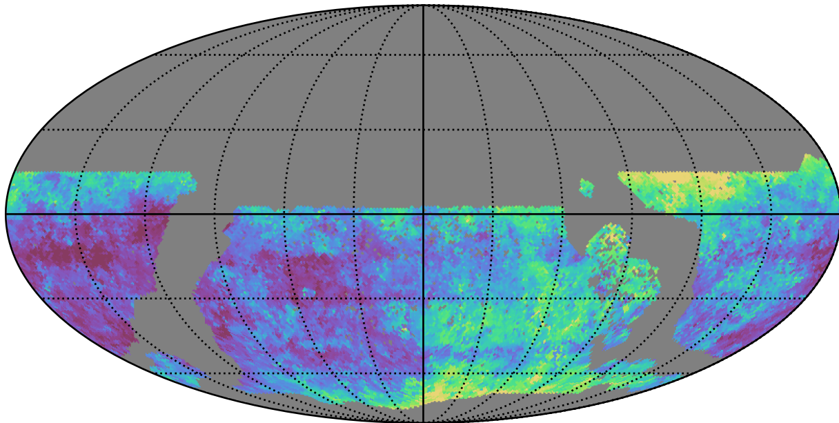
extra_ss_neo7_v3.4_10yrs WFD u band: Median seeingEff
