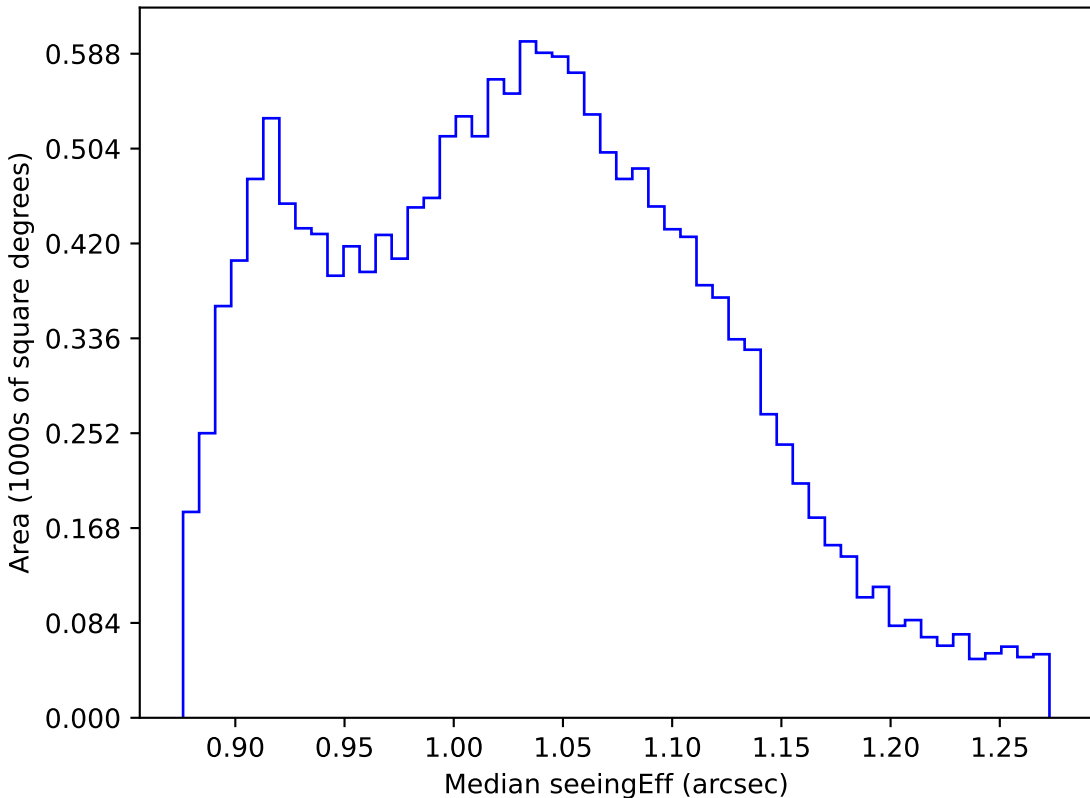
extra_ss_neo7_v3.4_10yrs WFD r band: Median seeingEff
