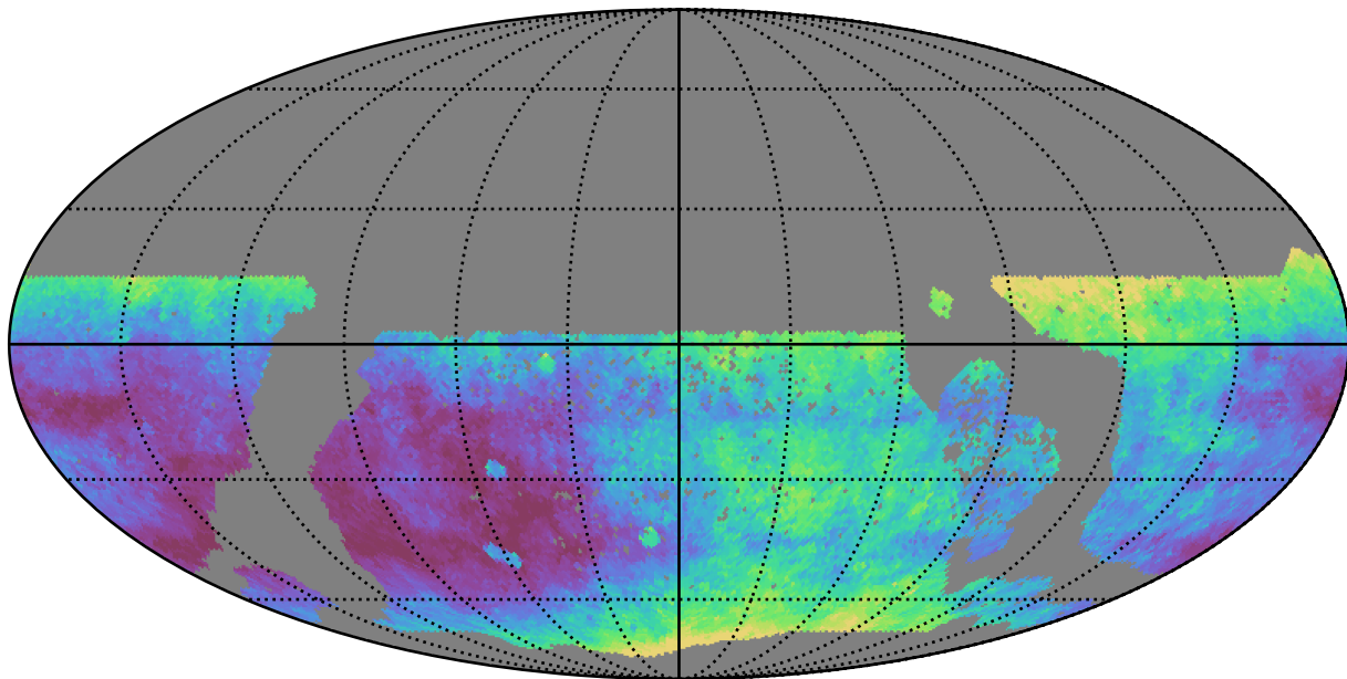
extra_ss_neo7_v3.4_10yrs WFD i band: Median seeingEff
