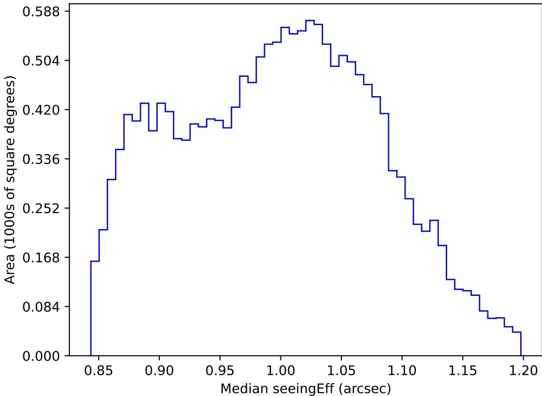
extra_ss_neo7_v3.4_10yrs WFD i band: Median seeingEff
