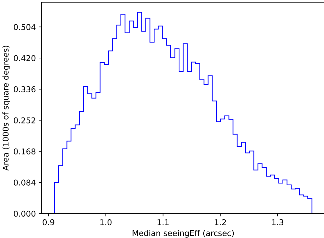
extra_ss_neo7_v3.4_10yrs WFD g band: Median seeingEff
