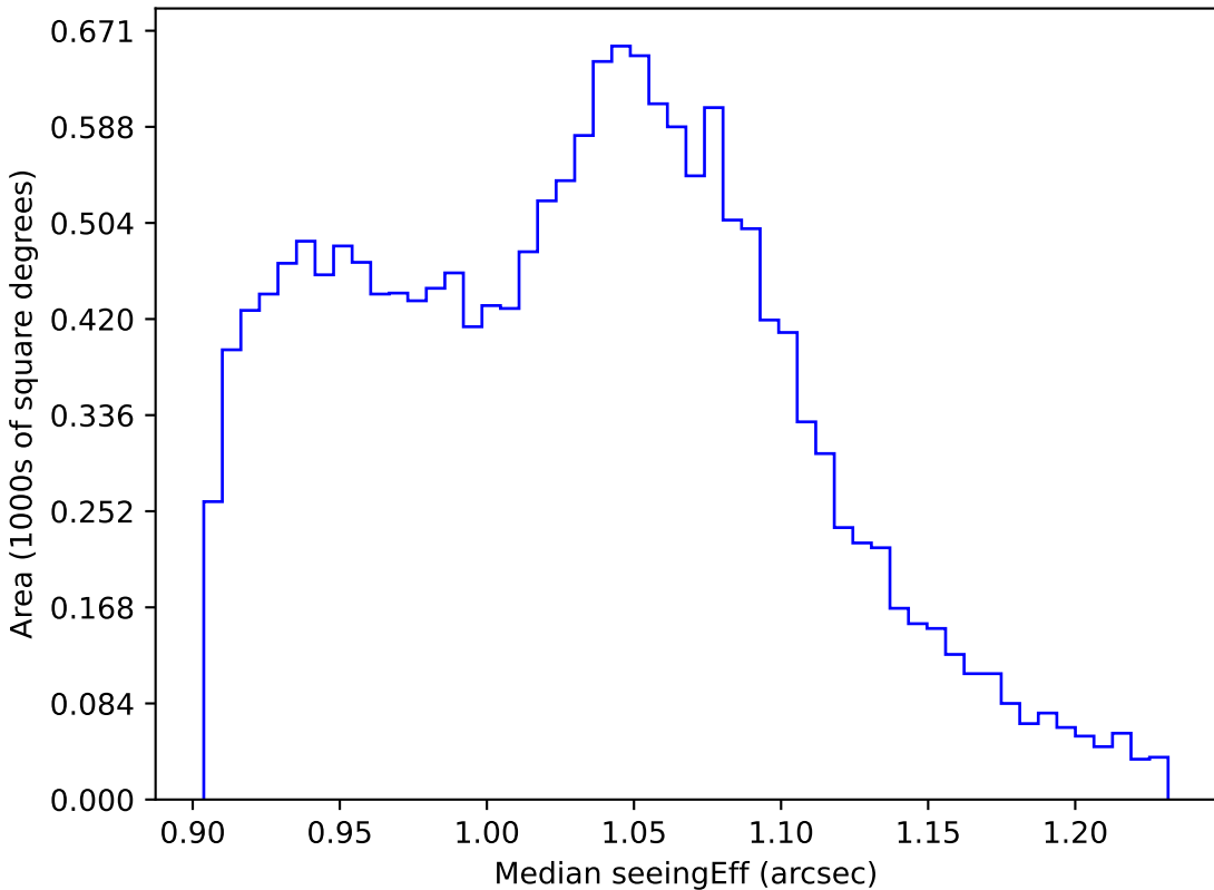
extra_ss_neo7_v3.4_10yrs WFD all bands: Median seeingEff
