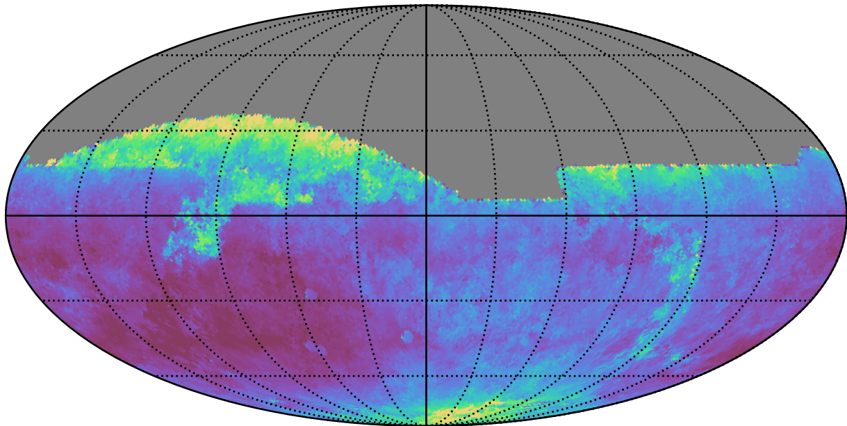
extra_ss_neo7_v3.4_10yrs All sky z band: Median seeingEff
