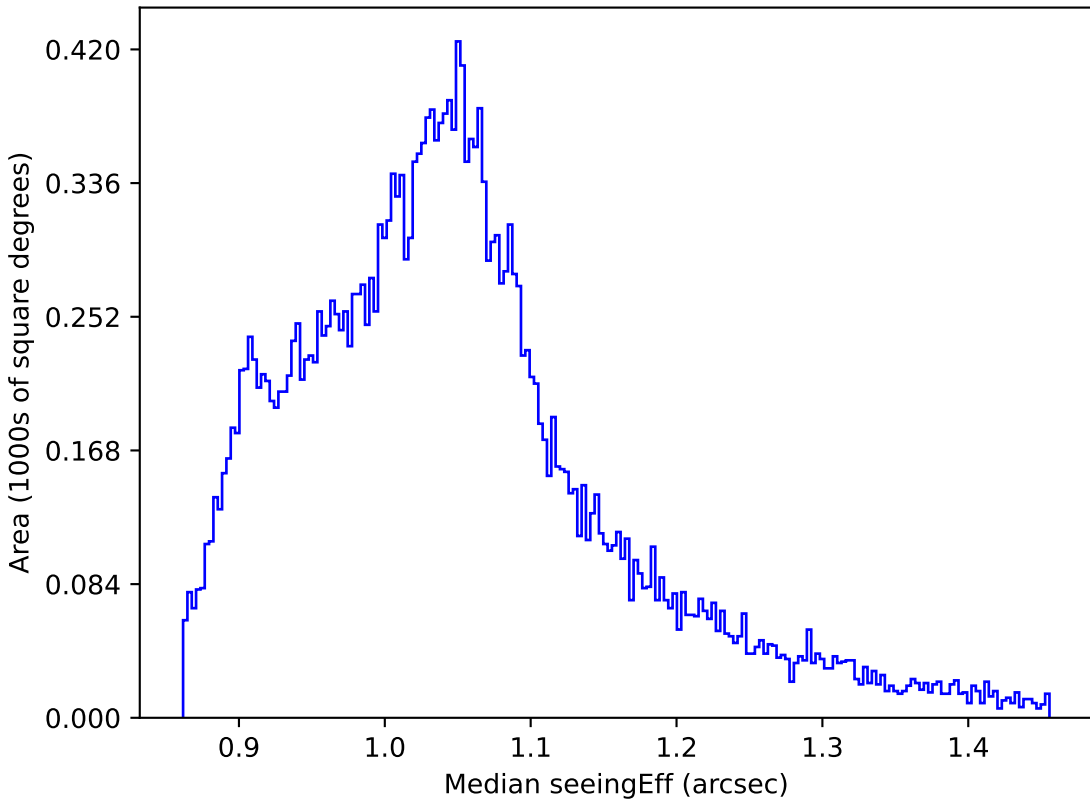
extra_ss_neo7_v3.4_10yrs All sky z band: Median seeingEff
