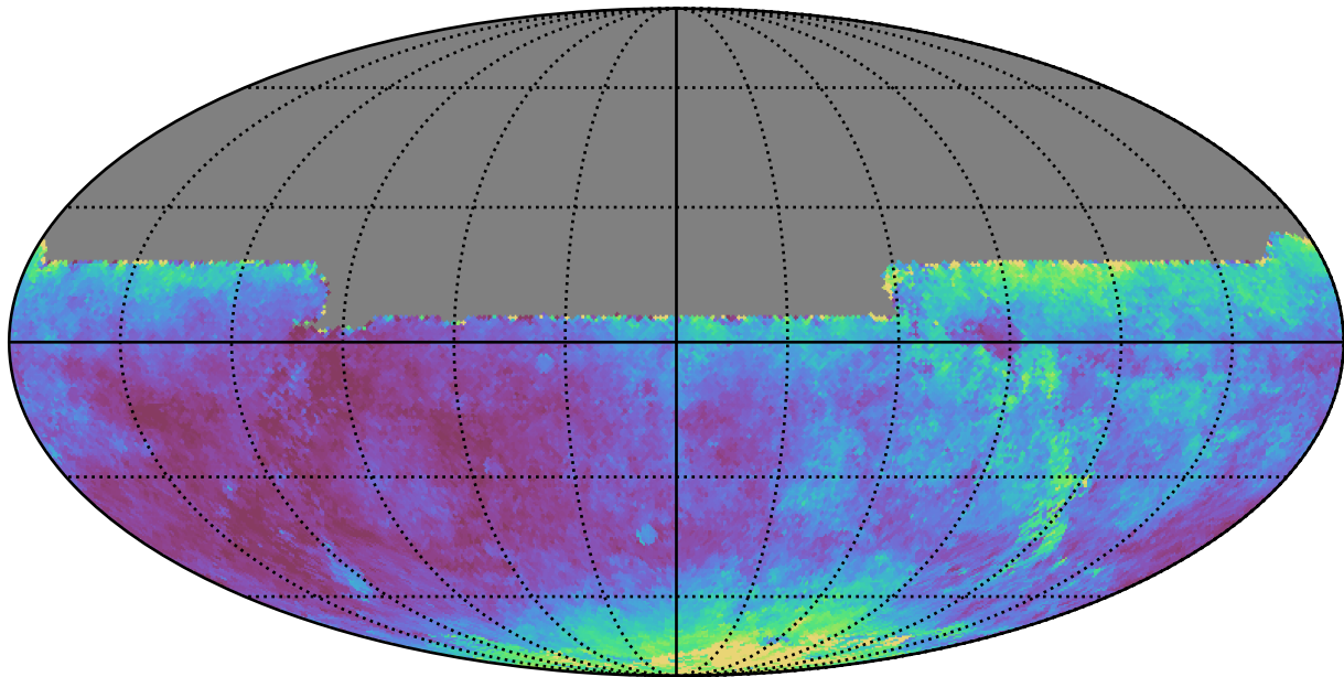
extra_ss_neo7_v3.4_10yrs All sky y band: Median seeingEff
