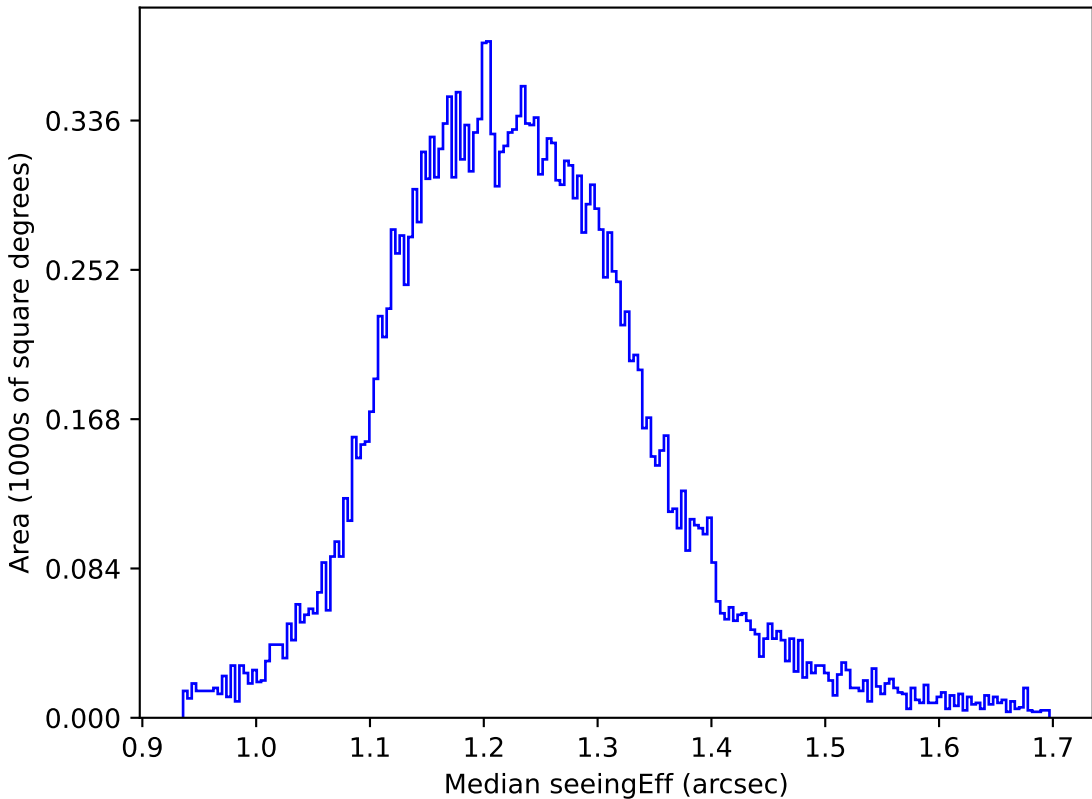
extra_ss_neo7_v3.4_10yrs All sky u band: Median seeingEff
