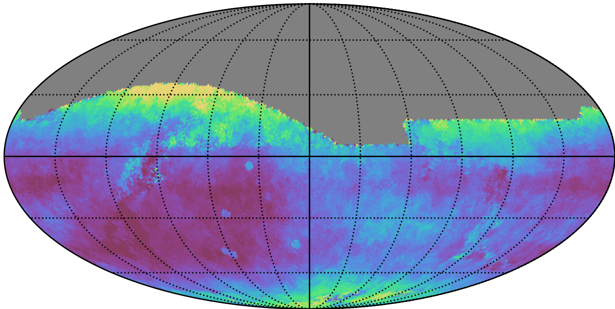
extra_ss_neo7_v3.4_10yrs All sky r band: Median seeingEff
