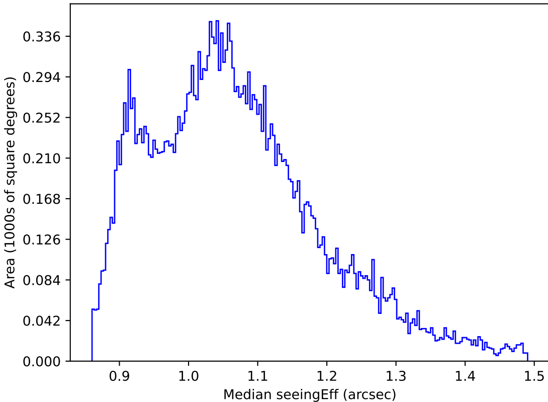
extra_ss_neo7_v3.4_10yrs All sky r band: Median seeingEff
