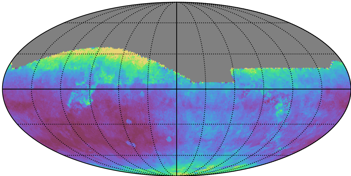
extra_ss_neo7_v3.4_10yrs All sky i band: Median seeingEff
