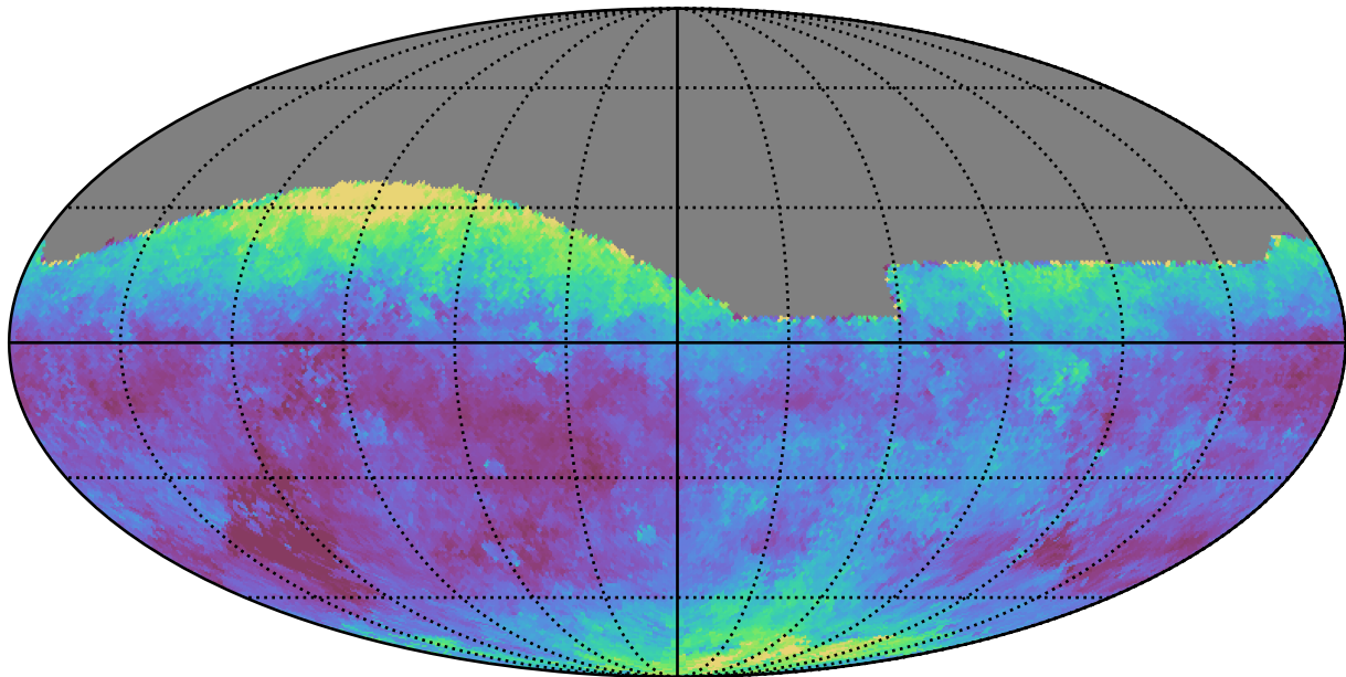
extra_ss_neo7_v3.4_10yrs All sky g band: Median seeingEff
