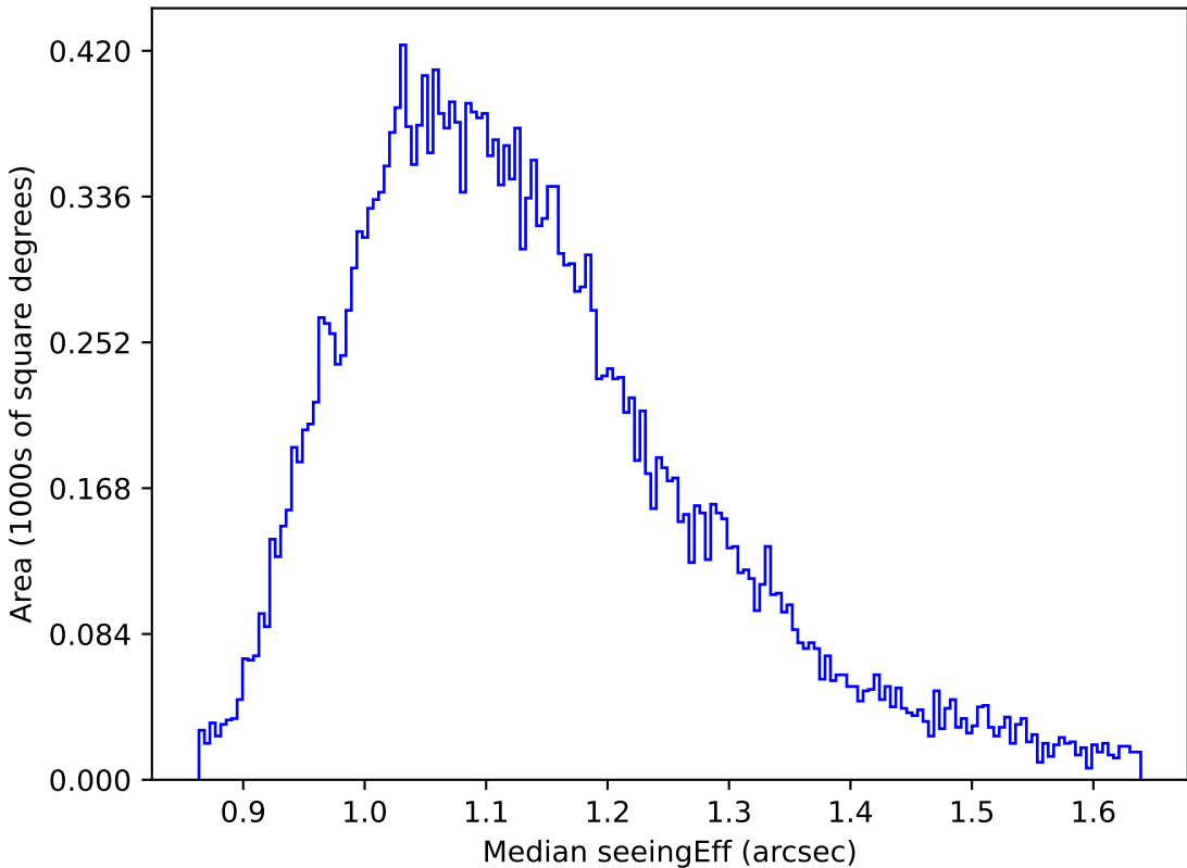
extra_ss_neo7_v3.4_10yrs All sky g band: Median seeingEff
