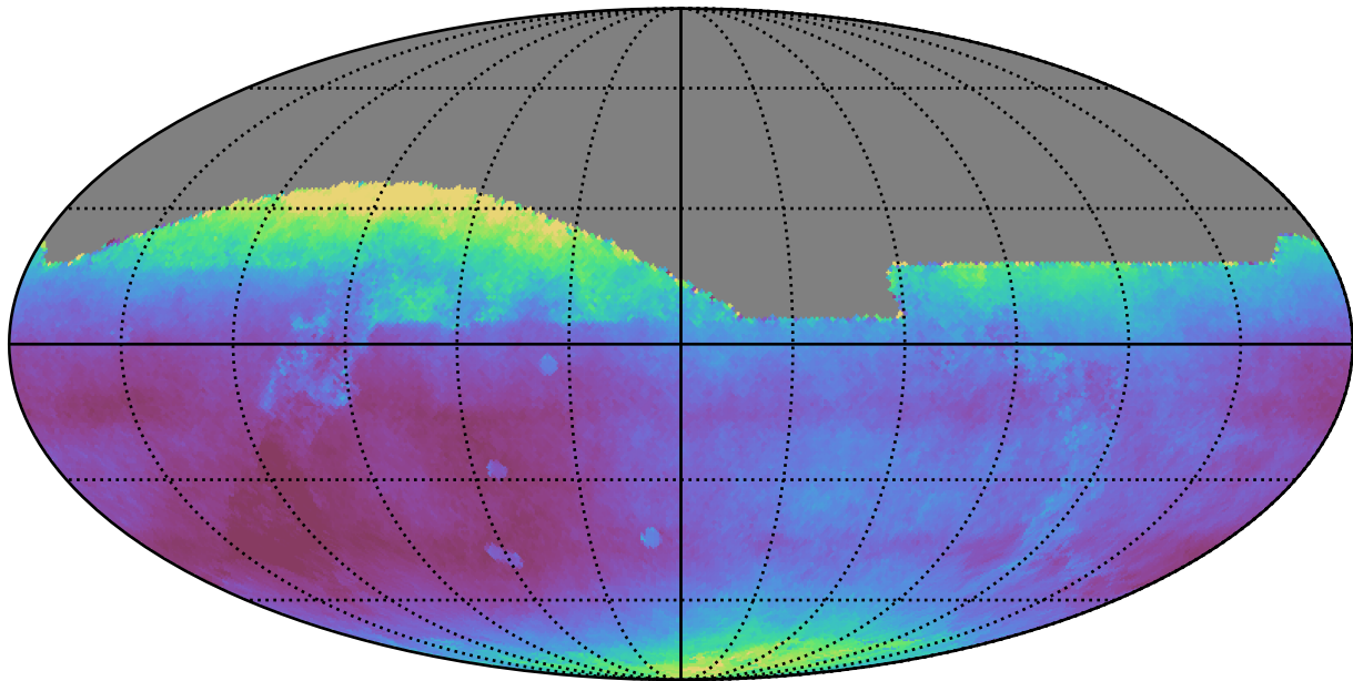
extra_ss_neo7_v3.4_10yrs All sky all bands: Median seeingEff
