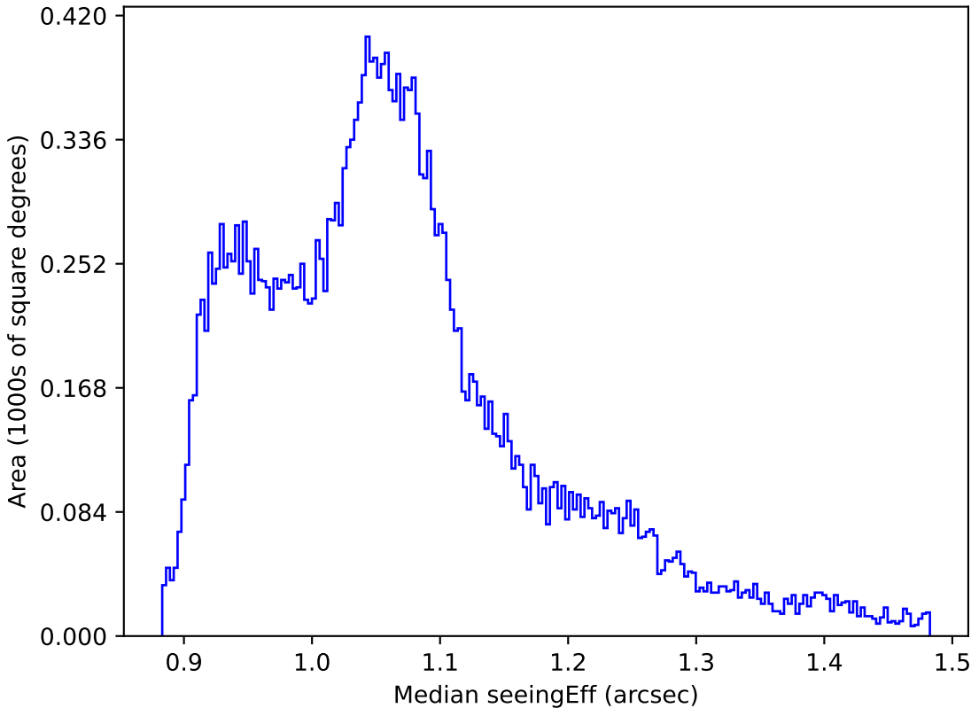
extra_ss_neo7_v3.4_10yrs All sky all bands: Median seeingEff
