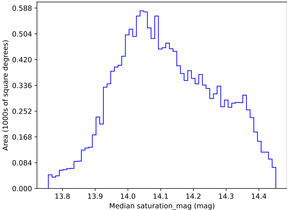
extra_ss_neo7_v3.4_10yrs WFD z band: Median saturation_mag
